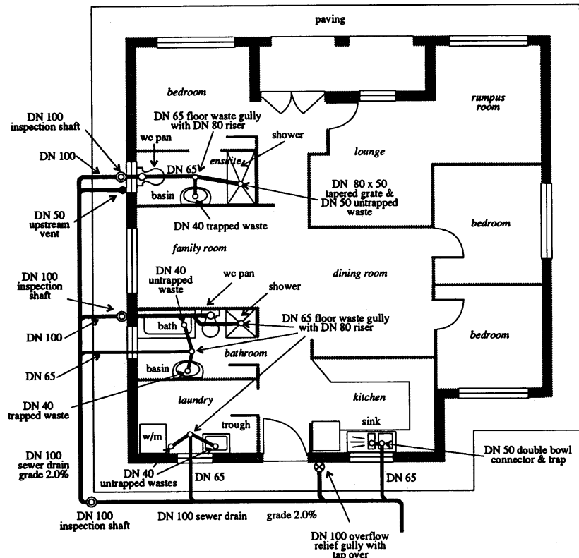
Figure 2: Building Layout Plan
